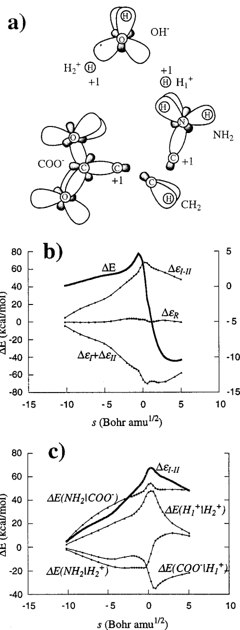
Figure 6. (a) Definition of the six functional groups of monohydrated glycine. (b) Energy components of the total energy along the reaction path of the gas phase water-assisted proton transfer: the barrier is due to the interaction term between the two simultaneous proton transfer processes. (c) Decomposition of the interaction energy in terms of its components: the energy of interaction of the \text{NH}_2 and \text{COO}^- groups and of the two protons dominates.
